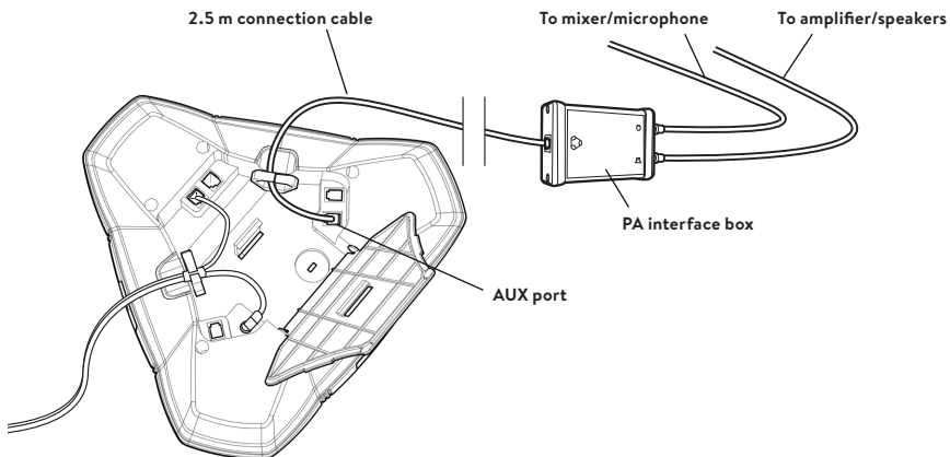
The picture shows the bottom of Konftel 300IP
